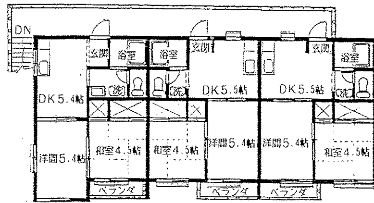
[2階平面図]
